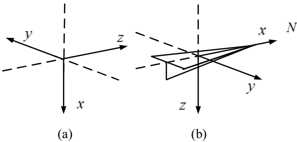
Fig.9: camera coordinate system and body coordinate system
