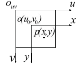
Fig. 6: Pixel coordinate system and image coordinate system
