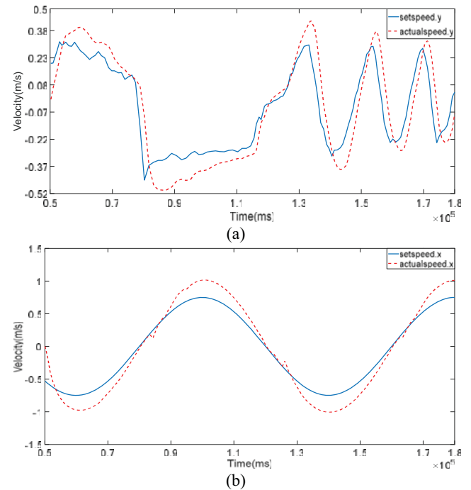
Fig. 10: Velocity response without PID control
