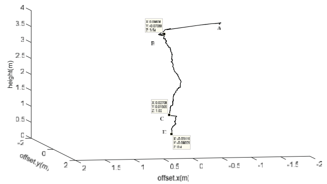
Fig.14: Landing trajectory
