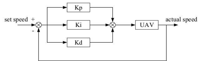
Fig.11 PID controller
