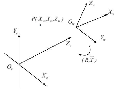
Fig. 7: World coordinate system and camera coordinate system
