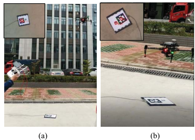
Fig. 3: The detection of AprilTags at different altitudes
