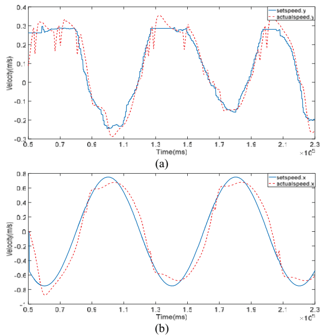
Fig.12: Velocity response with PID algorithm
