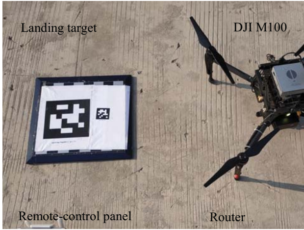
Fig. 4: System hardware
